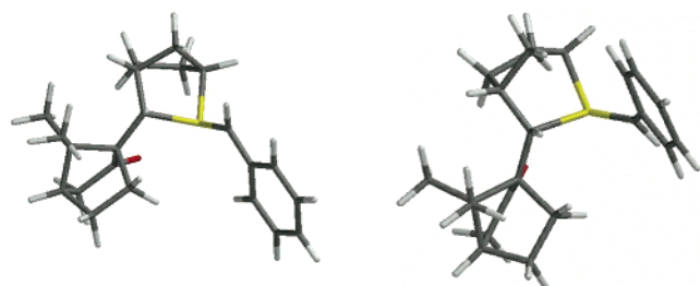
Figure 6. Models derived from DFT calculations showing the ylide conformations 8A and 8B , respectively.
