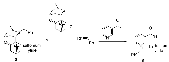
Scheme 4. Competitive Interception of Metal Carbenoid by Pyridyl Substrates
