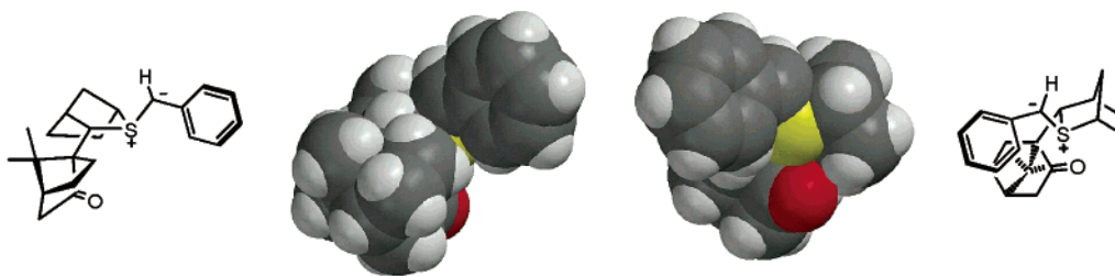
Figure 5. Space filling models derived from DFT calculations of 8A showing how the camphor group effectively blocks one face of the ylide from aldehyde attack. Related ChemDraw diagrams of the same view are given (for clarity).
