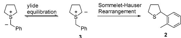
Scheme 3. Ylide Equilibration and Rearrangement
