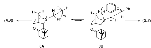
Scheme 6. Rationale for Enantioselectivity
