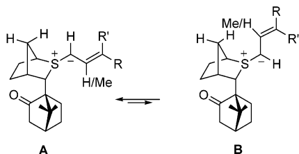
Scheme 9. Possible Conformers of \alpha,\beta -Unsaturated Sulfonium Ylides
